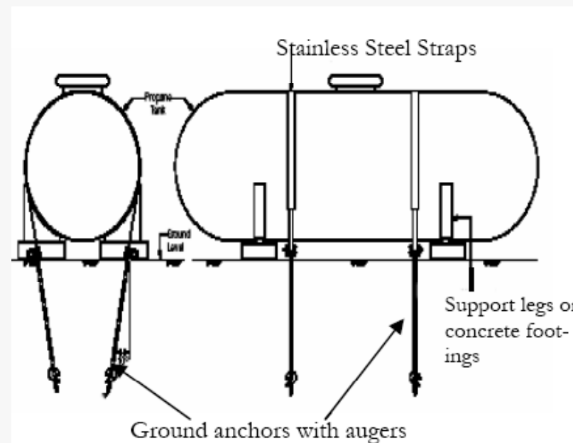
Ground Auger Installation
