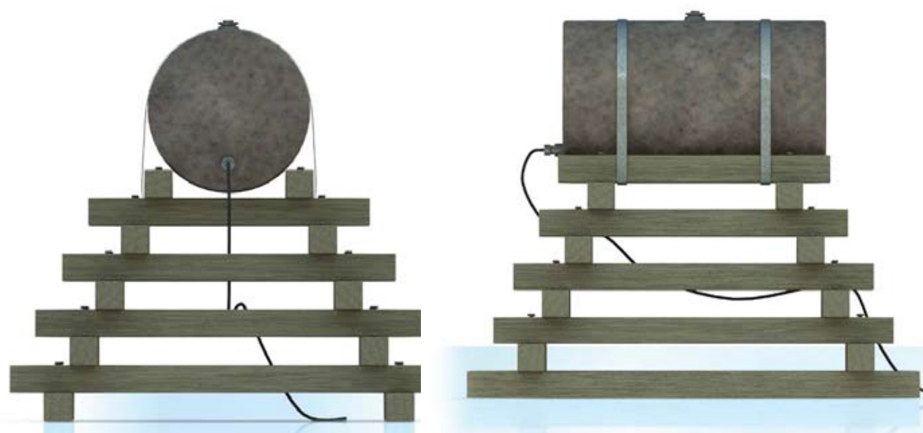
Timber Cradle Fuel Tank Stand
